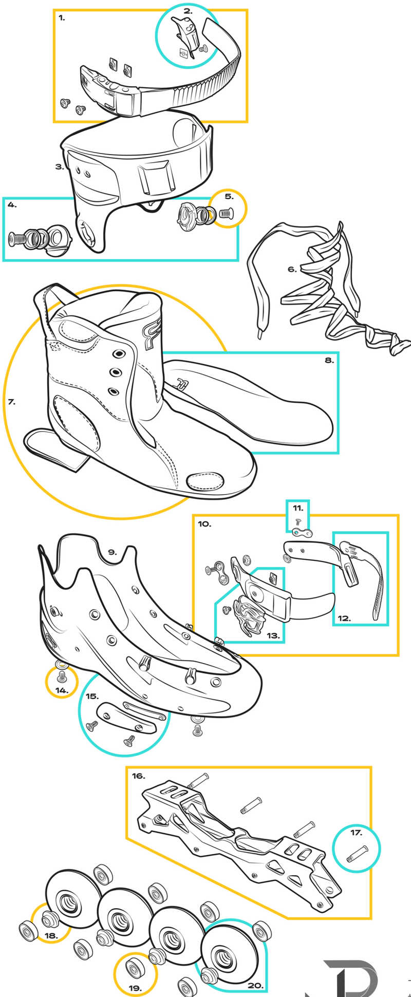
Exploded view - 2021 version
